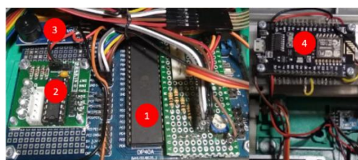
FIGURE 3. The module design of the device. (1) indicates microcontroller unit, (2) driver motor servo, (3) buzzer alarm, (4) Node MCU 8266.
