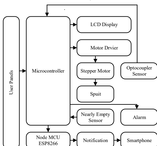
FIGURE 2. Block diagram of the experimental.
