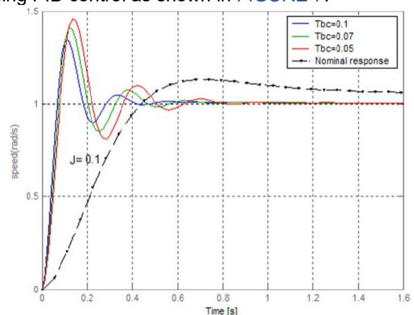
FIGURE 7. System Test Results with PID Controller
