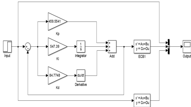
FIGURE 4. Simulink Block Eddy Current Brakes Dynamometer System with PID Control
