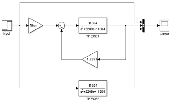
FIGURE 5. Simulink Block Eddy Current Brakes Dynamometer System with LQR Control
