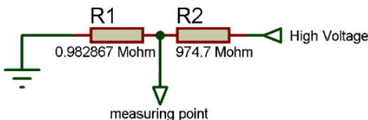
FIGURE 5. Measurement Circuit
