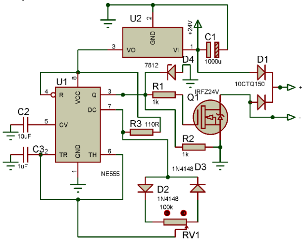
FIGURE 2. PWM Controller
