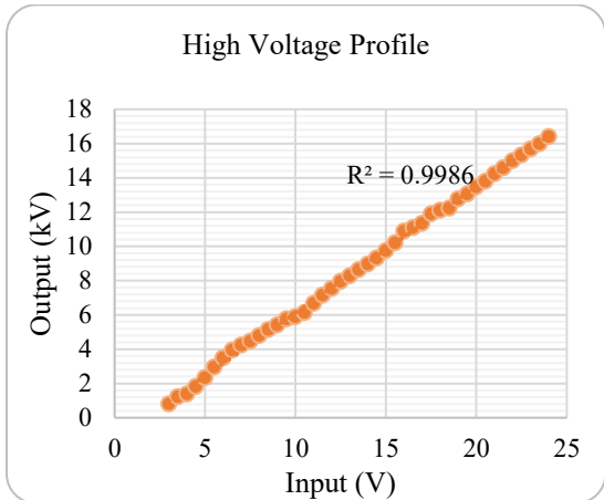
FIGURE 13. Output vs input linearity intended that high voltage is the robust condition
