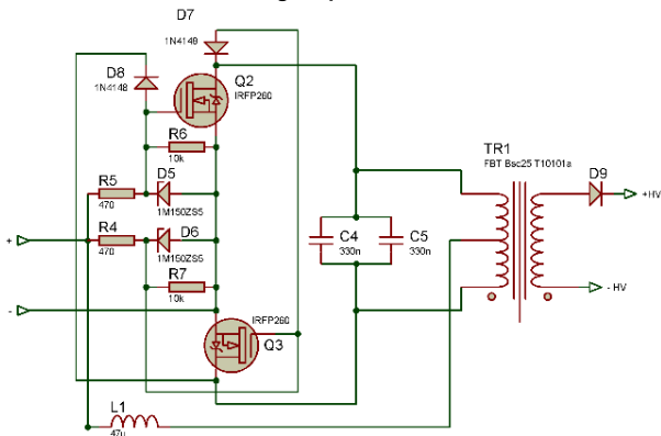
FIGURE 4. Mazzili ZVS Flyback Converter
