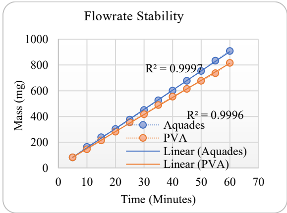
FIGURE 12. Linearity flowrate indicates that flowrate is stable
