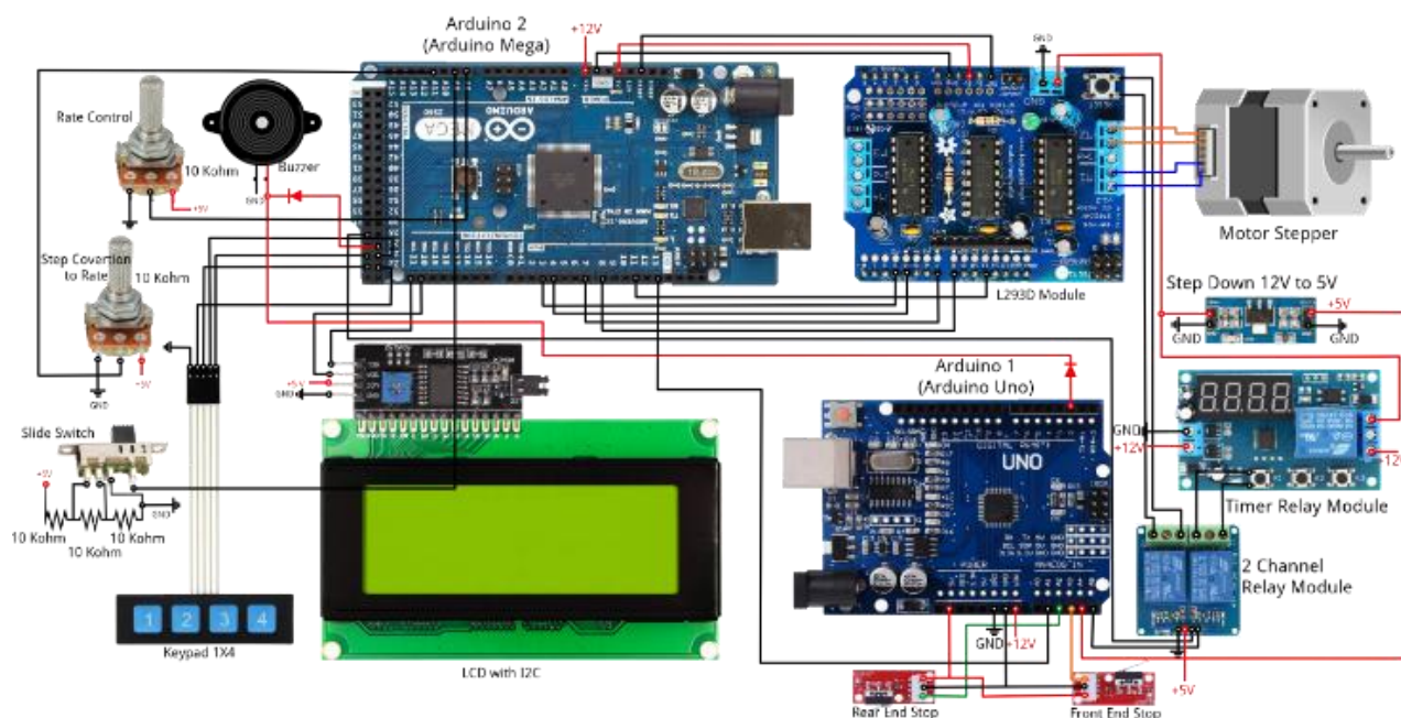
FIGURE 1. Schematic Design of The Syringe Pump
