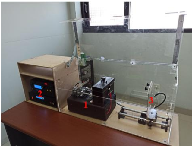
FIGURE 7. The Electrospinning Machine
