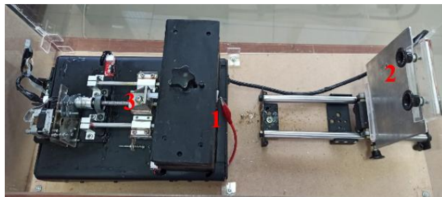
FIGURE 8. Syringe Pump and Collector System
