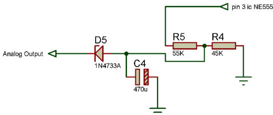
FIGURE 3. Analog Output to Microcontroller
