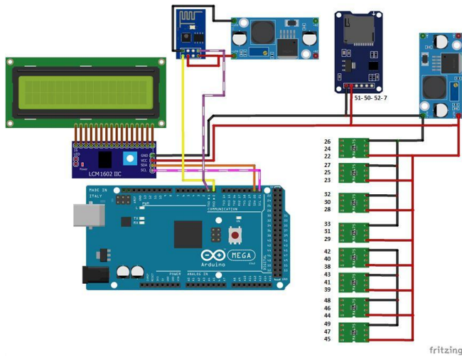
FIGURE 2. Thermocouple system circuit
