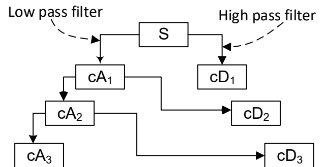
FIGURE 3. Details Coefficient and Aproximation Coefficient from Discrete Wavelet Transform Decomposition
