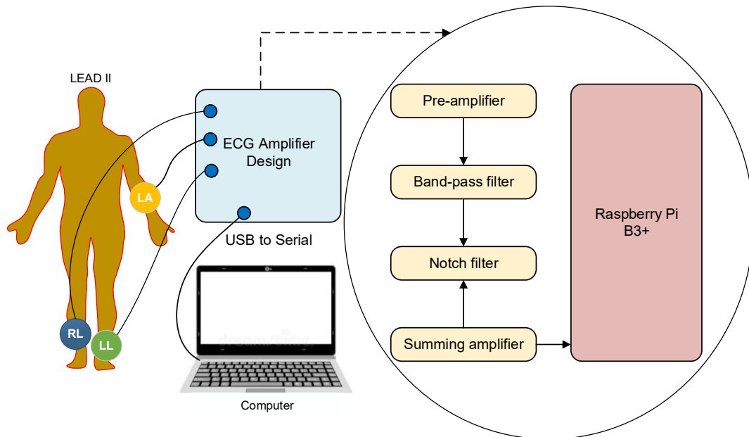
FIGURE 2. System Diagram Blocks. When the system is turned on, the voltage on the patient electrode will be tapped and processed on the ECG Module. The Raspberry microcontroller will process the ECG signal from the ECG Module. Then the data will be processed and displayed on the PC
