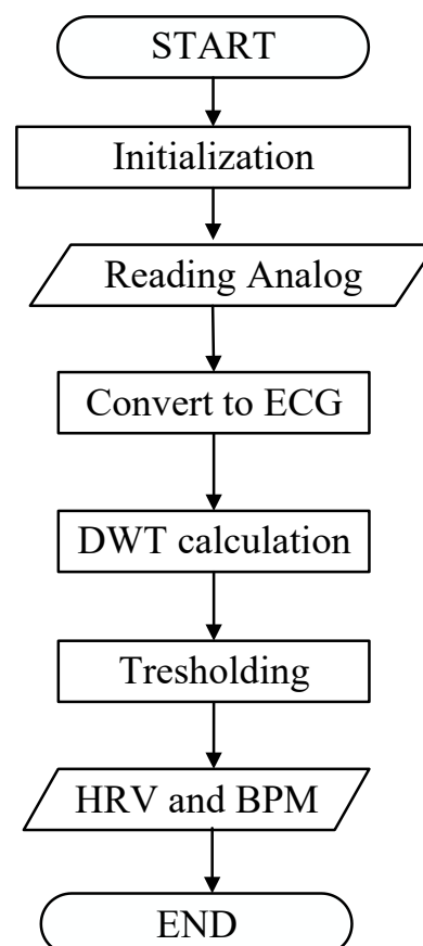
FIGURE 1. Flow chart of how the system works from the beginning to read the ADC value until it is processed and produces HRV and BPM values.
