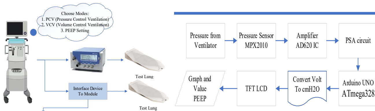
FIGURE 1. Block Diagram of Flow Analyzer Module
