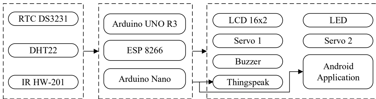
FIGURE 1. Diagram block of medical box system
