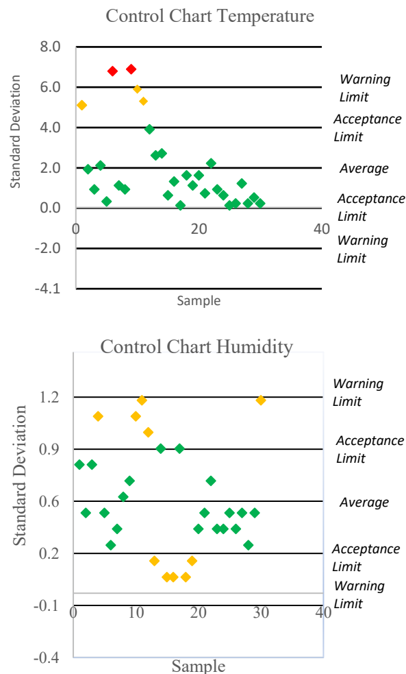
FIGURE 6. Graph of Precision Standard Deviation of Temperature and Humidity
