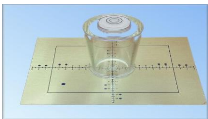
FIGURE 4. Visualization of how the beam alignment and collimator test tool is placed above the x-ray tube on the bucky table.
