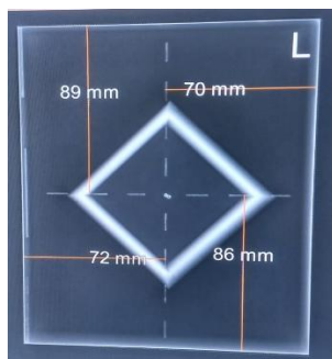
FIGURE 8. Results of the collimation test on a phillips x-ray machine, the value of the light lap for x1 is 7 cm, x2 is 7 cm, y1 is 9 cm, and y2 is 9 cm. Then for the value of the x-ray lap, x1 is obtained 7cm, for x2 7.2 cm, for y1 8.6 cm, for y2 8.9 cm.
