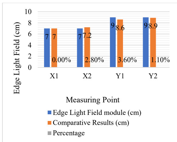
FIGURE 5. Chart contains of module results to the results of x-ray images perpendicular conditions.
