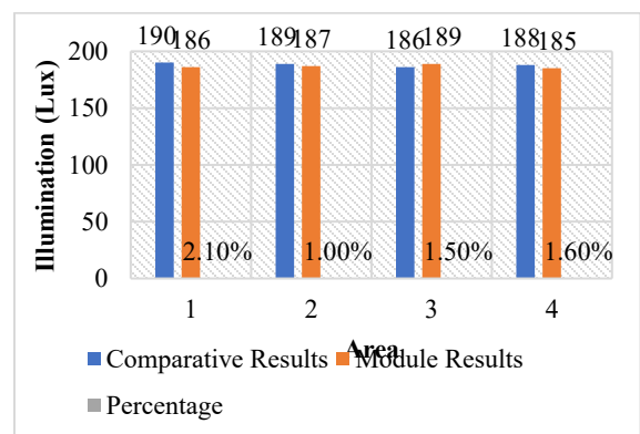
FIGURE 3. Chart contains of the Illumination measurement result Measurements were made by comparing the module with the Digital Light Meter Model 5202 KYORITSU ELECTRICAL INSTRUMENTS WORKS, LTD.
