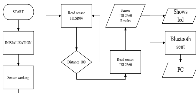
FIGURE 2. Flowchart containing the tool workflow from the tool on to completion.
