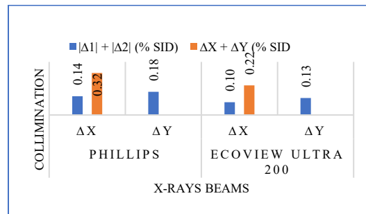
FIGURE 7. Results of the collimation field difference test with X-Ray Beams.
