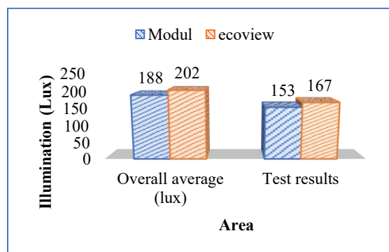
FIGURE 6. Chart contains of x-ray modality collimator light Illumination test results by comparing overall average with light room measurements.
