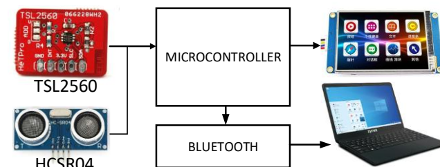
FIGURE 1. Block diagram contains input, process, and output blocks
