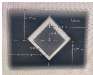
FIGURE 9. Collimation test results on the ecoview ultra 200 x-ray machine, the value of the light lap for x1 is 7 cm, x2 is 7 cm, y1 is 9 cm, and y2 is 9 cm. Then the x-ray values are obtained for x1 6.7 cm, x2 values are 7.1 cm, y1 values 9.4 cm, and y2 values 9.08 cm.
