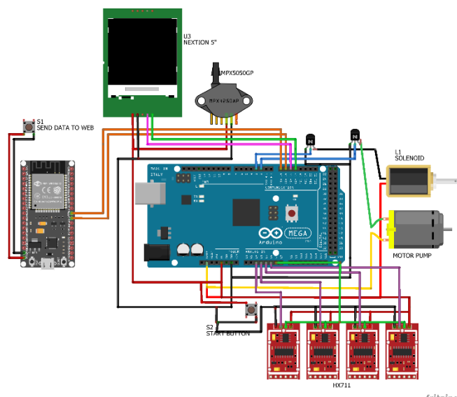
FIGURE 4. Bed ANC system circuit for operating device Bed ANC for Preecalmsi
