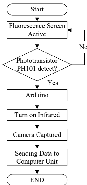
FIGURE 2. Flowchart of the digital detector
