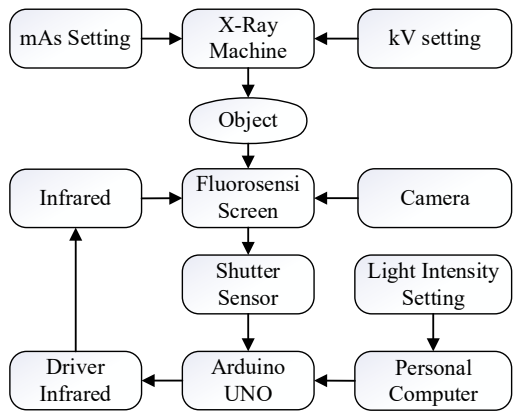
FIGURE 1. The diagram block of digital detector
